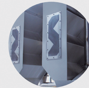
Zig-zag Classifier
